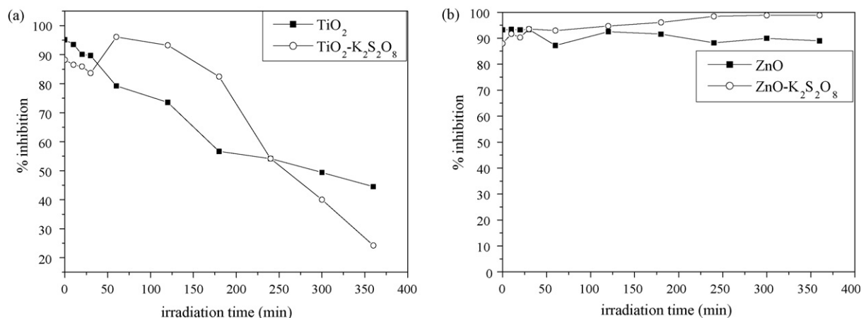
Fig. 8. Toxicity evolution as a function of irradiation time in the presence of: (a) TiO_2 = 100 \text{ mg L}^{-1} , TiO_2 = 100 \text{ mg L}^{-1} + K_2S_2O_8 = 3.1 \text{ mM} and (b) ZnO = 500 \text{ mg L}^{-1} , ZnO = 500 \text{ mg L}^{-1} + K_2S_2O_8 = 3.1 \text{ mM} .
