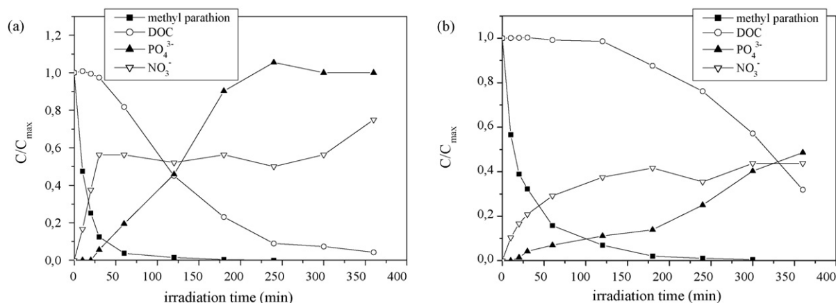
Fig. 7. Parathion/DOC reduction and PO_4^{3-}/NO_3^- release as a function of irradiation time, methyl parathion = 25 \text{ mg L}^{-1} : (a) TiO_2 = 100 \text{ mg L}^{-1} , K_2S_2O_8 = 3.1 \text{ mM} and (b) ZnO = 500 \text{ mg L}^{-1} , K_2S_2O_8 = 3.1 \text{ mM} .
